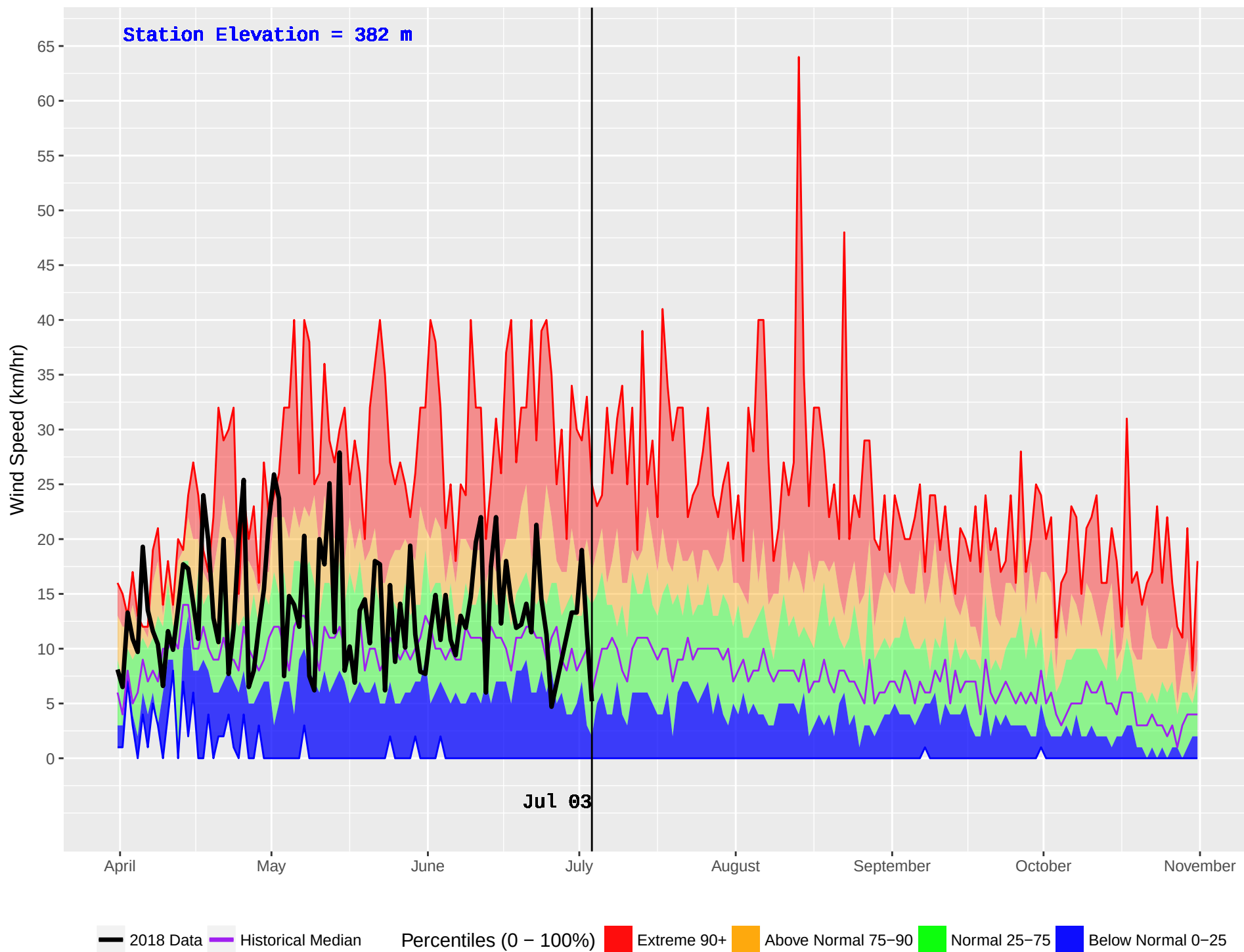
TELEGRAPH CREEK (110) : Historical (1978–2016) and Current (2018) Noon Wind Speed
